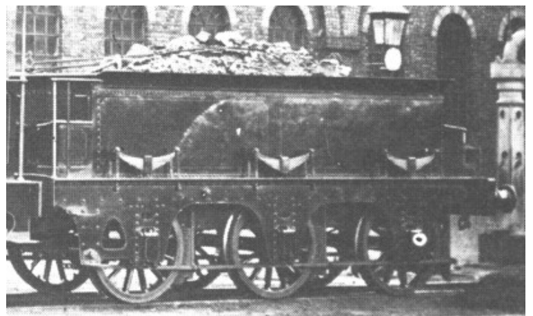
Belgravia's early tender: large open frame
