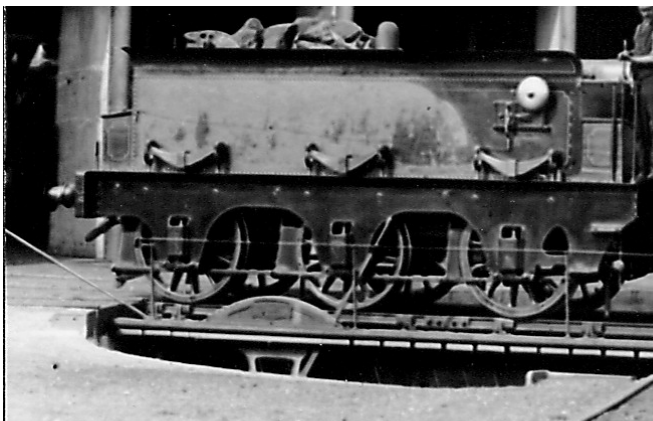
Carisbrooke's tender: large open frame
