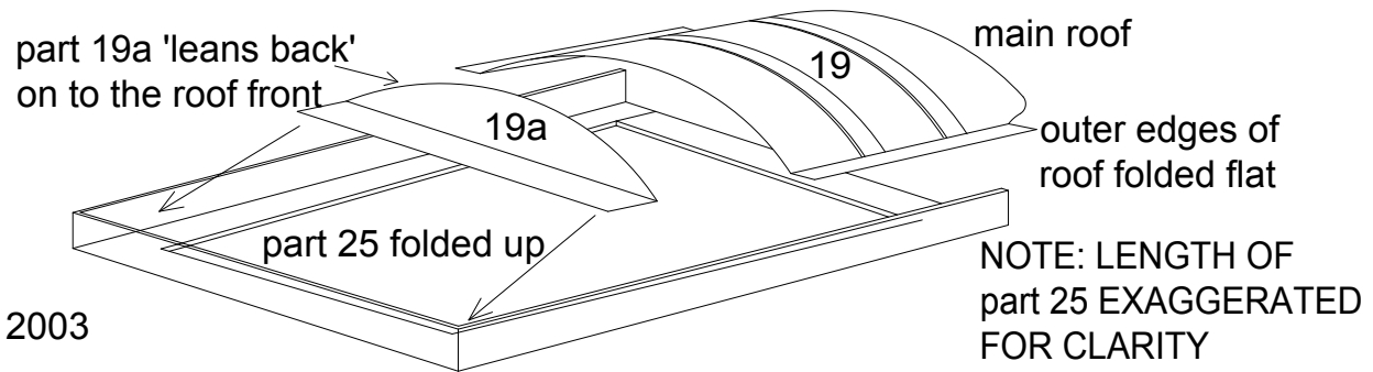
Diagram 13 Roof construction
