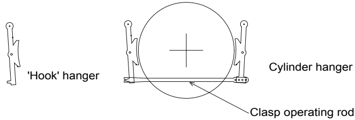
Diagram 6 Brakes: schematic Arrangement
